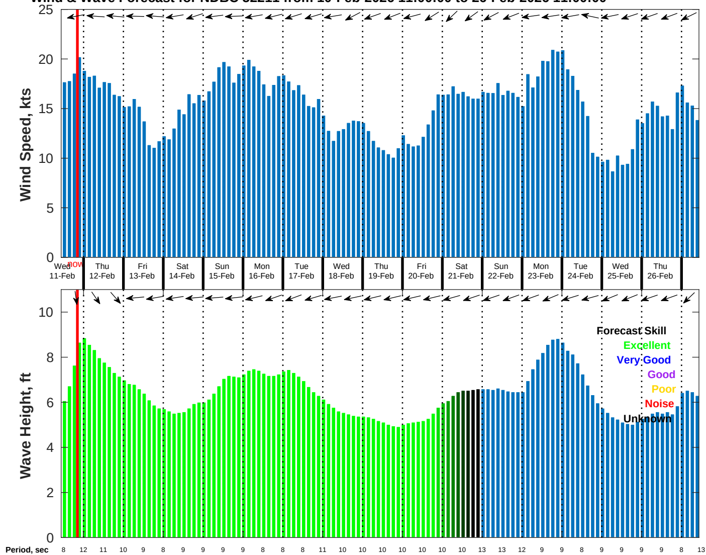
Wind & Wave Forecast for NDBC 52211 from 10-Feb-2026 11:00:00 to 26-Feb-2026 11:00:00
