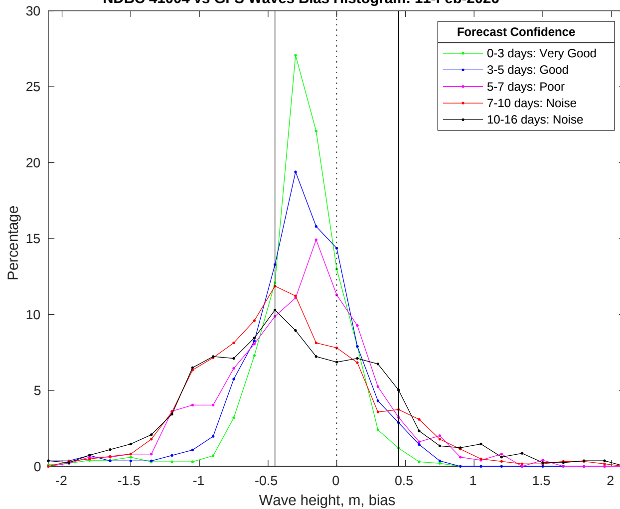
NDBC 41004 vs GFS Waves Bias Histogram: 11-Feb-2026
