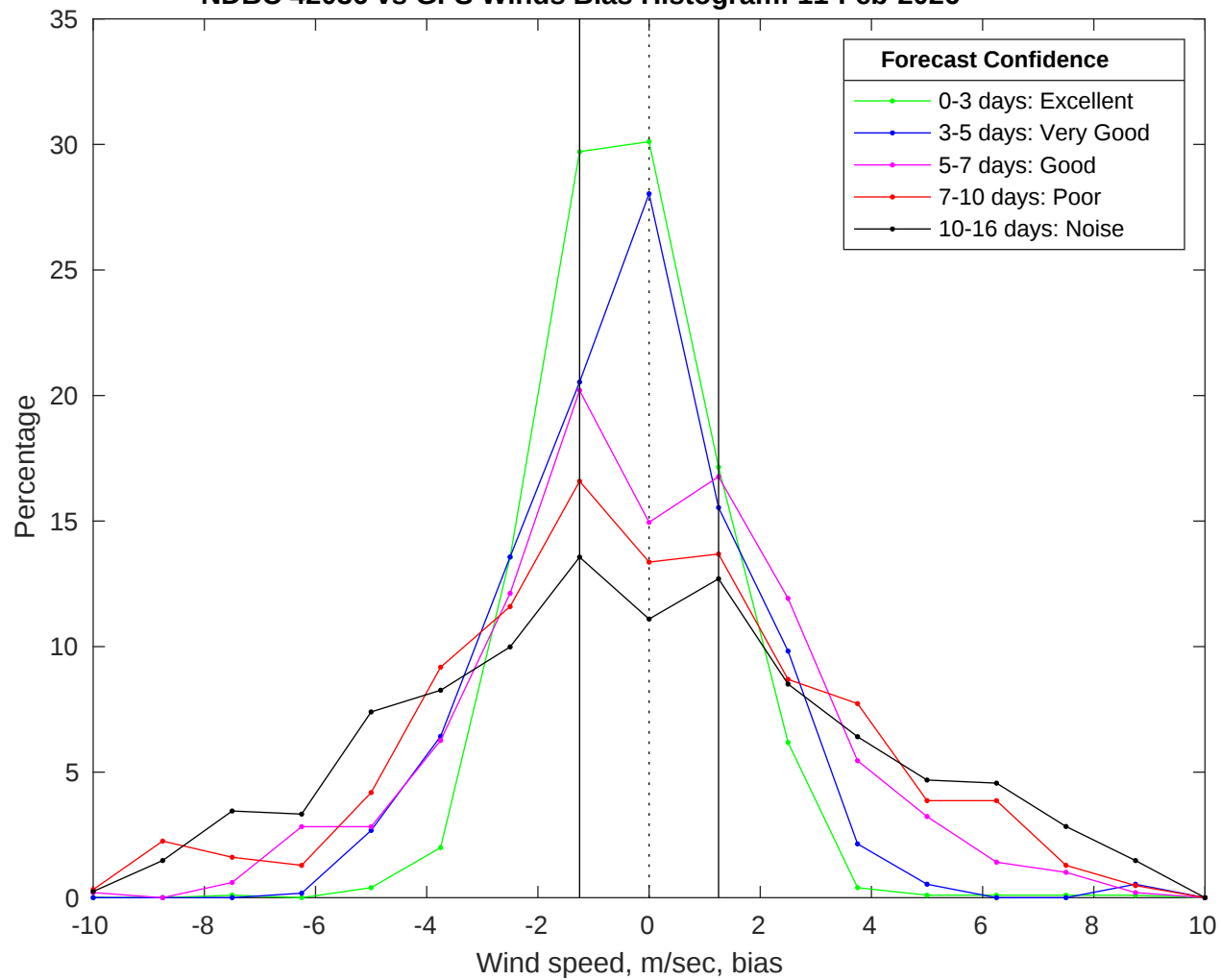
NDBC 42036 vs GFS Winds Bias Histogram: 11-Feb-2026
