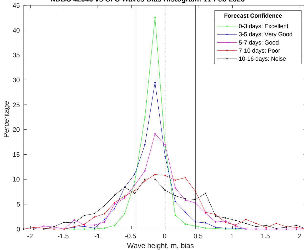
NDBC 42040 vs GFS Waves Bias Histogram: 11-Feb-2026
