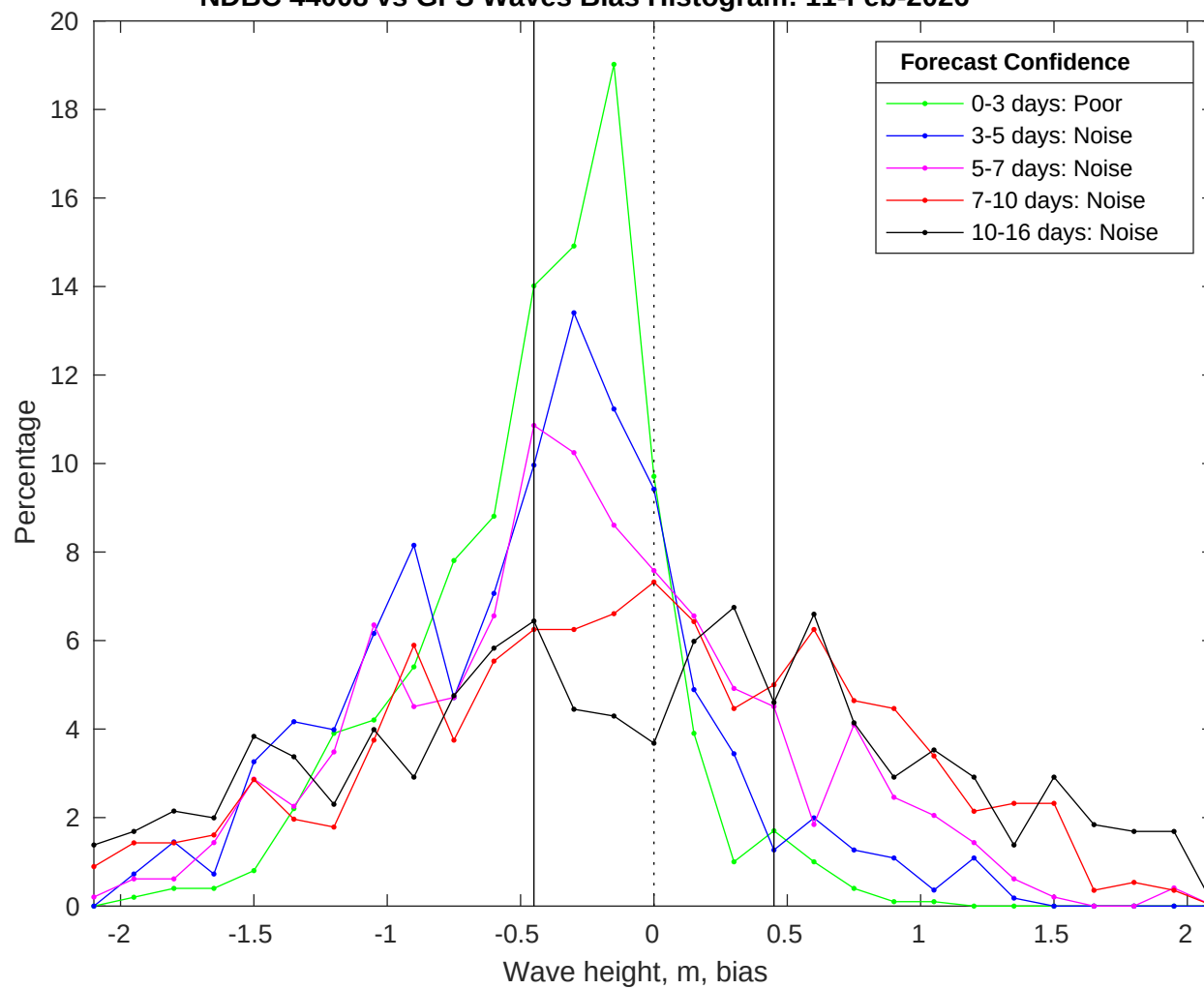
NDBC 44008 vs GFS Waves Bias Histogram: 11-Feb-2026
