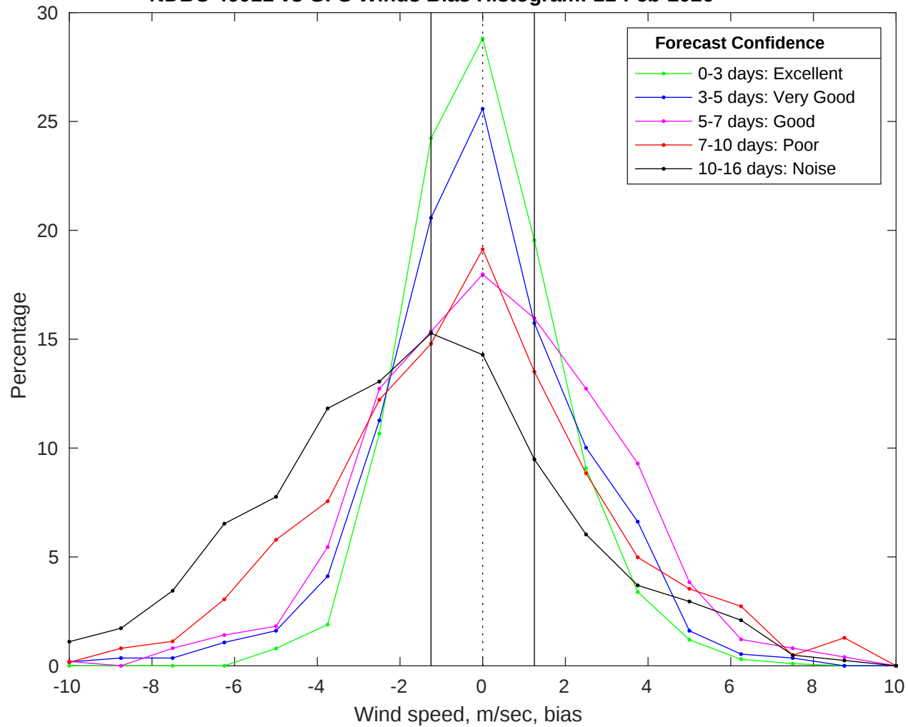
NDBC 46011 vs GFS Winds Bias Histogram: 11-Feb-2026
