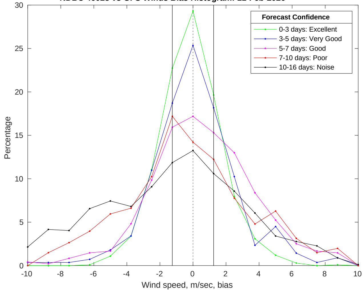
NDBC 46028 vs GFS Winds Bias Histogram: 11-Feb-2026
