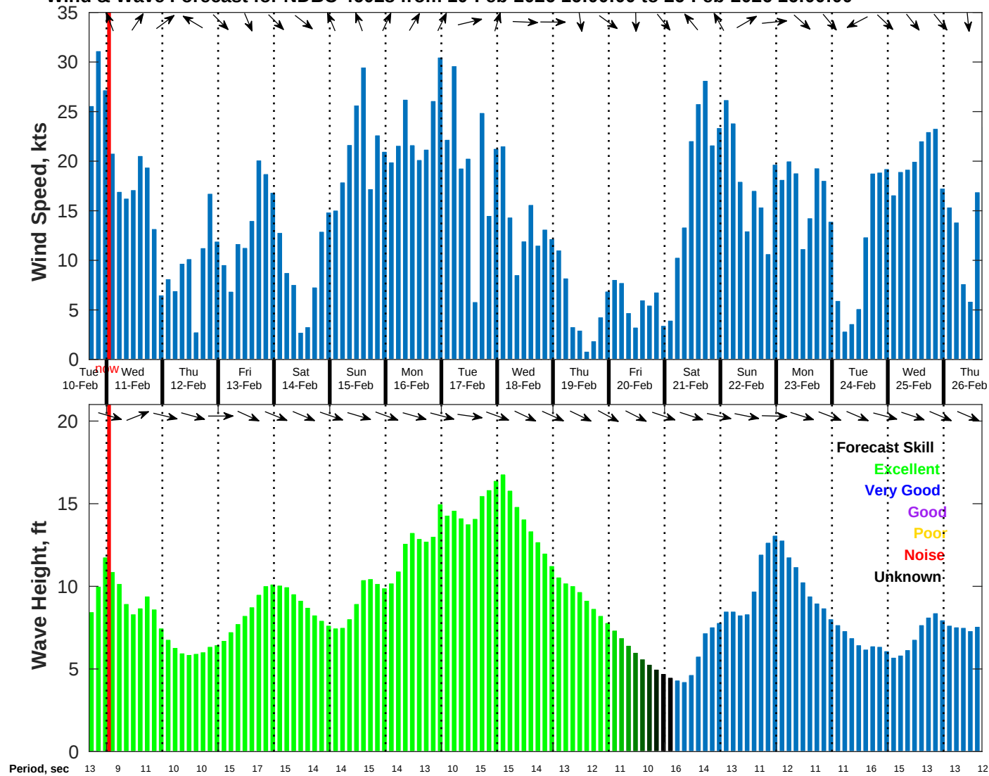
Wind & Wave Forecast for NDBC 46028 from 10-Feb-2026 16:00:00 to 26-Feb-2026 16:00:00
