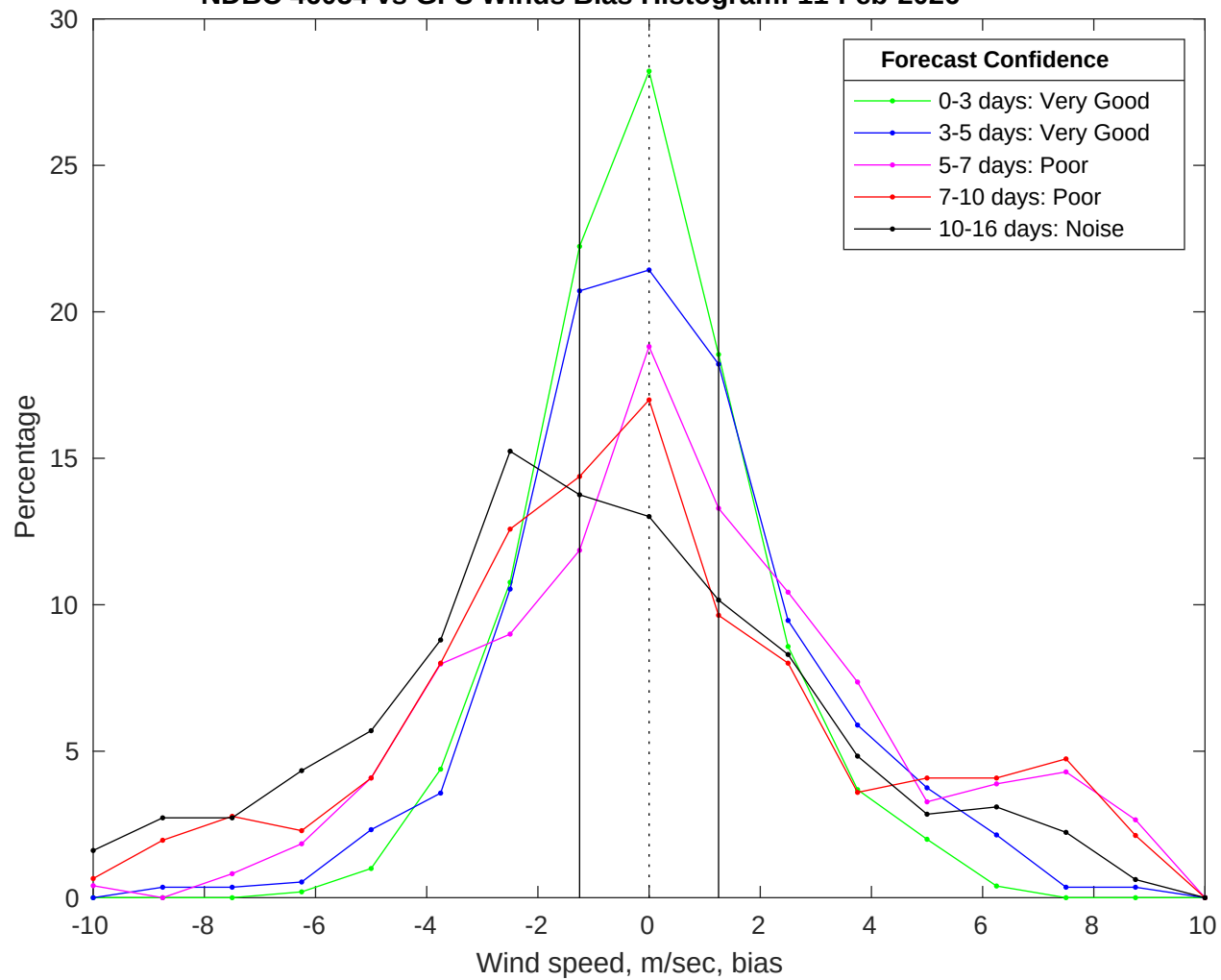
NDBC 46054 vs GFS Winds Bias Histogram: 11-Feb-2026
