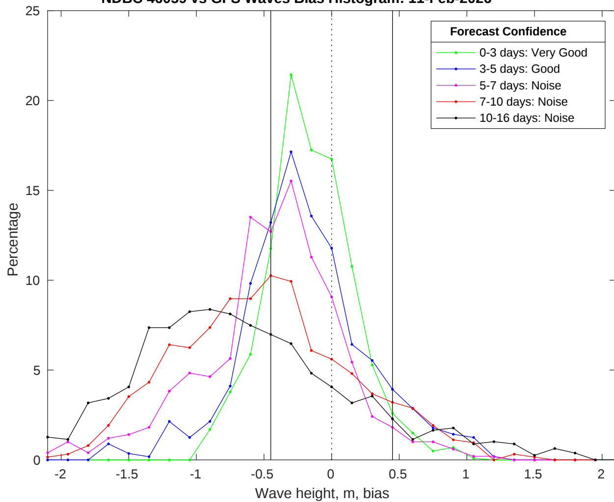
NDBC 46059 vs GFS Waves Bias Histogram: 11-Feb-2026
