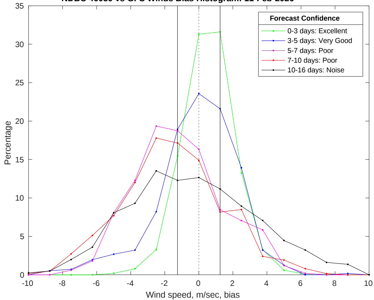
NDBC 46059 vs GFS Winds Bias Histogram: 11-Feb-2026
