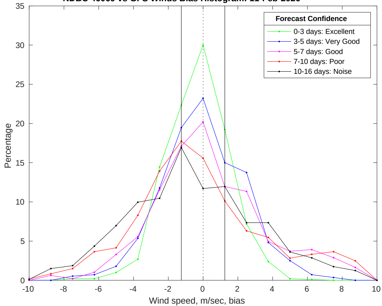
NDBC 46069 vs GFS Winds Bias Histogram: 11-Feb-2026
