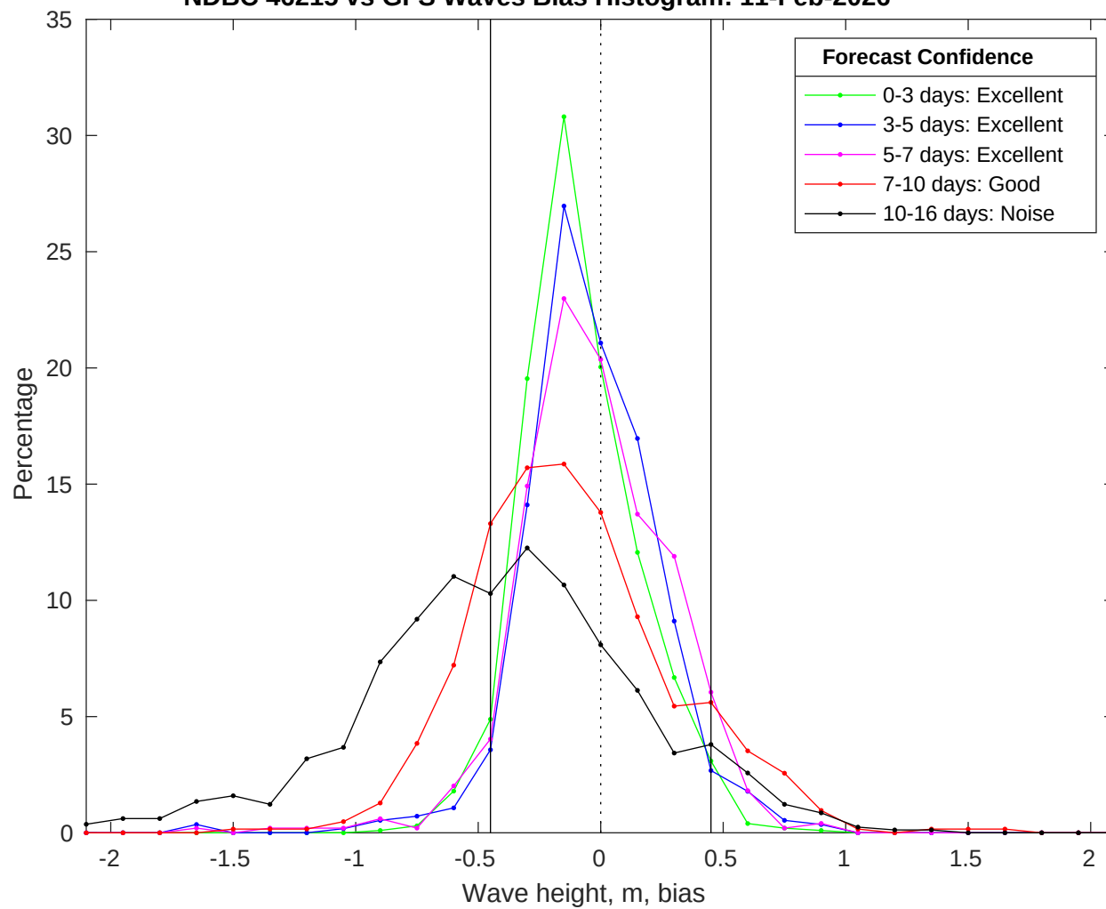
NDBC 46215 vs GFS Waves Bias Histogram: 11-Feb-2026
