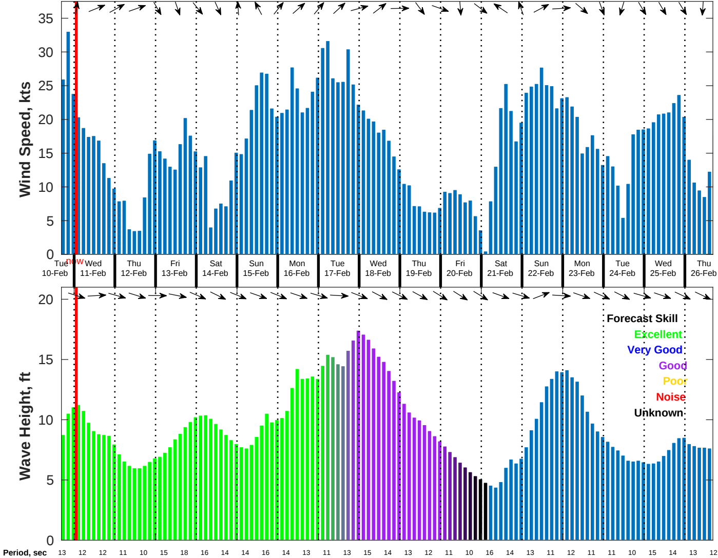
Wind & Wave Forecast for NDBC 46259 from 10-Feb-2026 16:00:00 to 26-Feb-2026 16:00:00
