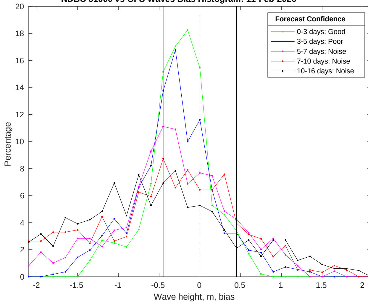
NDBC 51000 vs GFS Waves Bias Histogram: 11-Feb-2026
