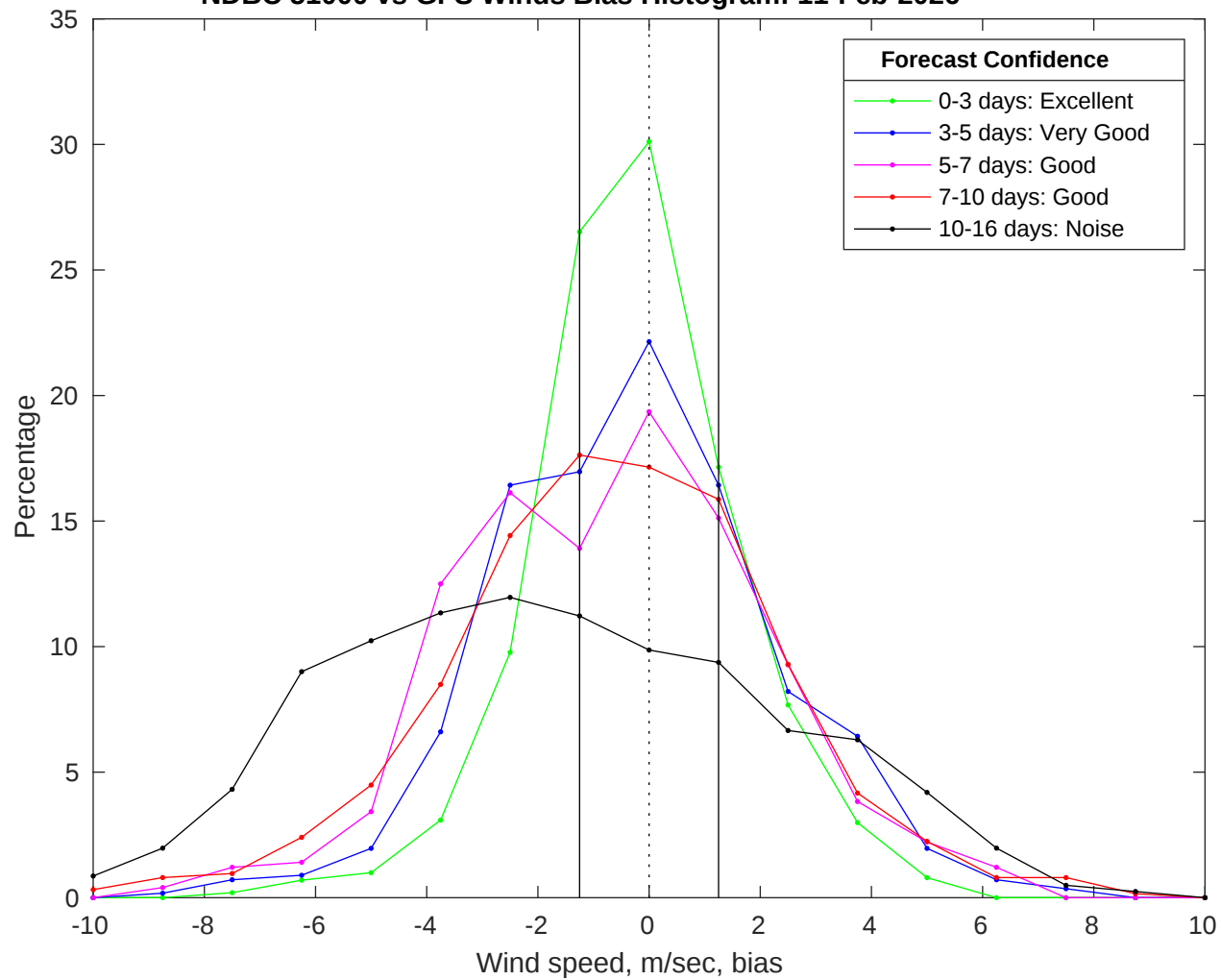
NDBC 51000 vs GFS Winds Bias Histogram: 11-Feb-2026
