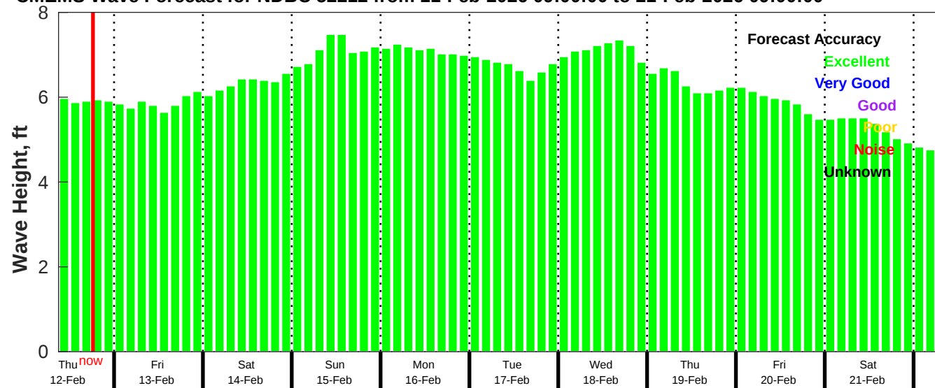
CMEMS Wave Forecast for NDBC 52212 from 11-Feb-2026 09:00:00 to 21-Feb-2026 09:00:00
