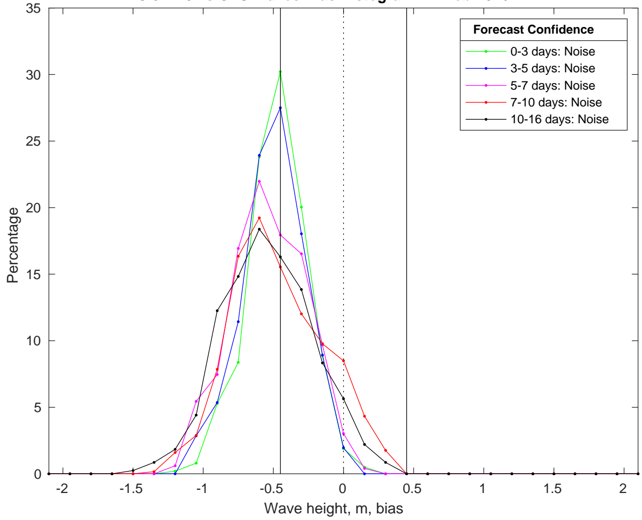
NDBC 52213 vs GFS Waves Bias Histogram: 11-Feb-2026
