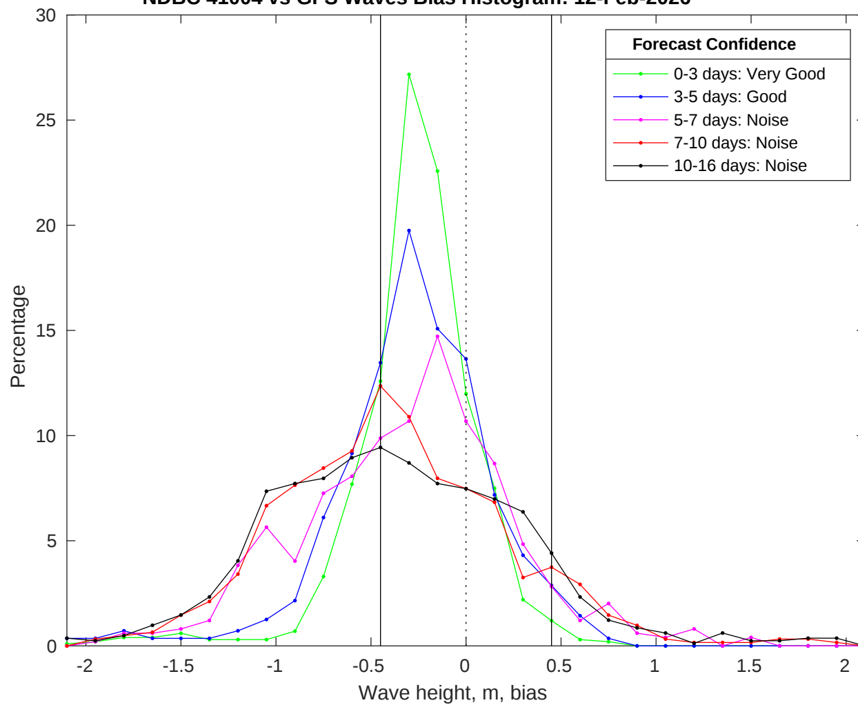
NDBC 41004 vs GFS Waves Bias Histogram: 12-Feb-2026
