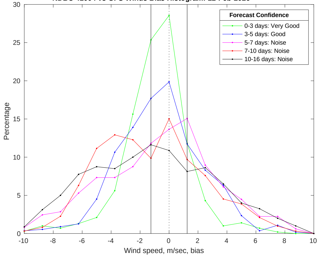
NDBC 41004 vs GFS Winds Bias Histogram: 12-Feb-2026
