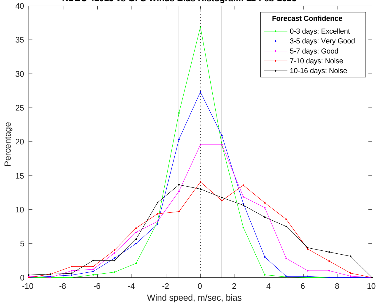
NDBC 42019 vs GFS Winds Bias Histogram: 12-Feb-2026
