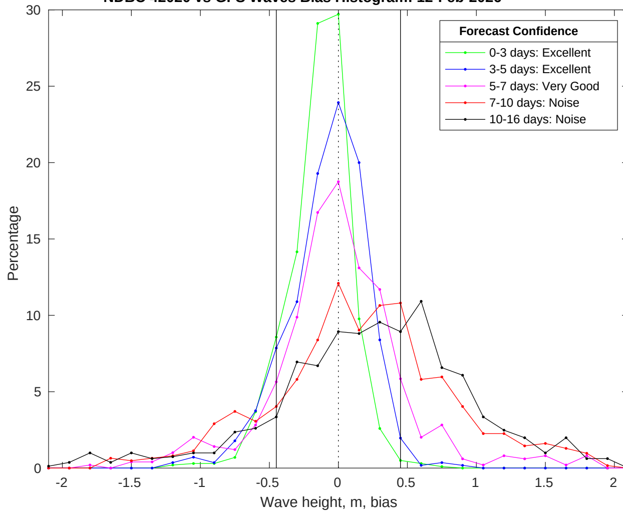
NDBC 42020 vs GFS Waves Bias Histogram: 12-Feb-2026
