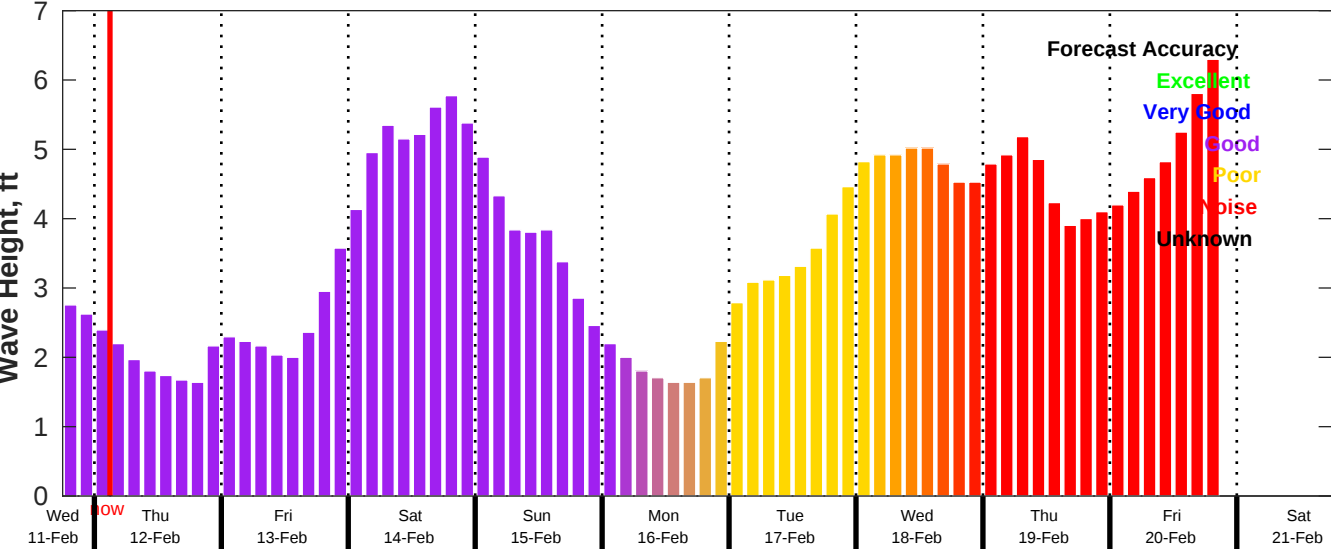
CMEMS Wave Forecast for NDBC 42020 from 11-Feb-2026 18:00:00 to 21-Feb-2026 18:00:00
