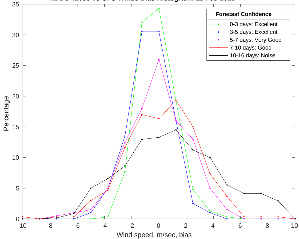
NDBC 42035 vs GFS Winds Bias Histogram: 12-Feb-2026
