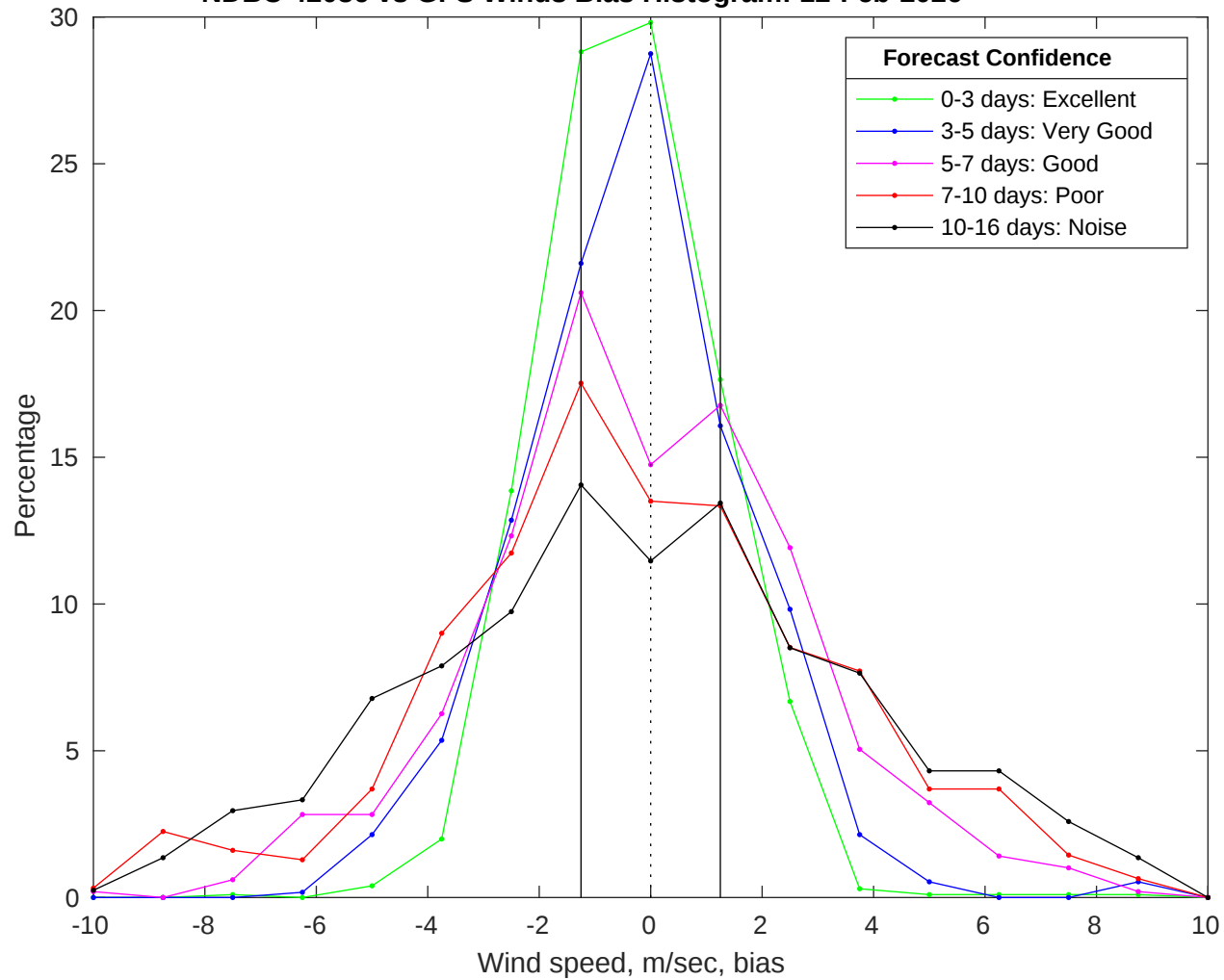
NDBC 42036 vs GFS Winds Bias Histogram: 12-Feb-2026
