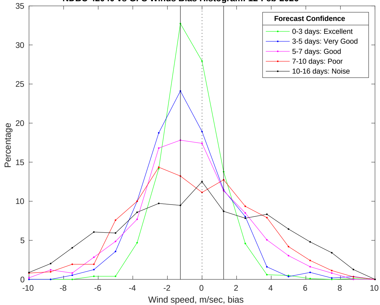
NDBC 42040 vs GFS Winds Bias Histogram: 12-Feb-2026
