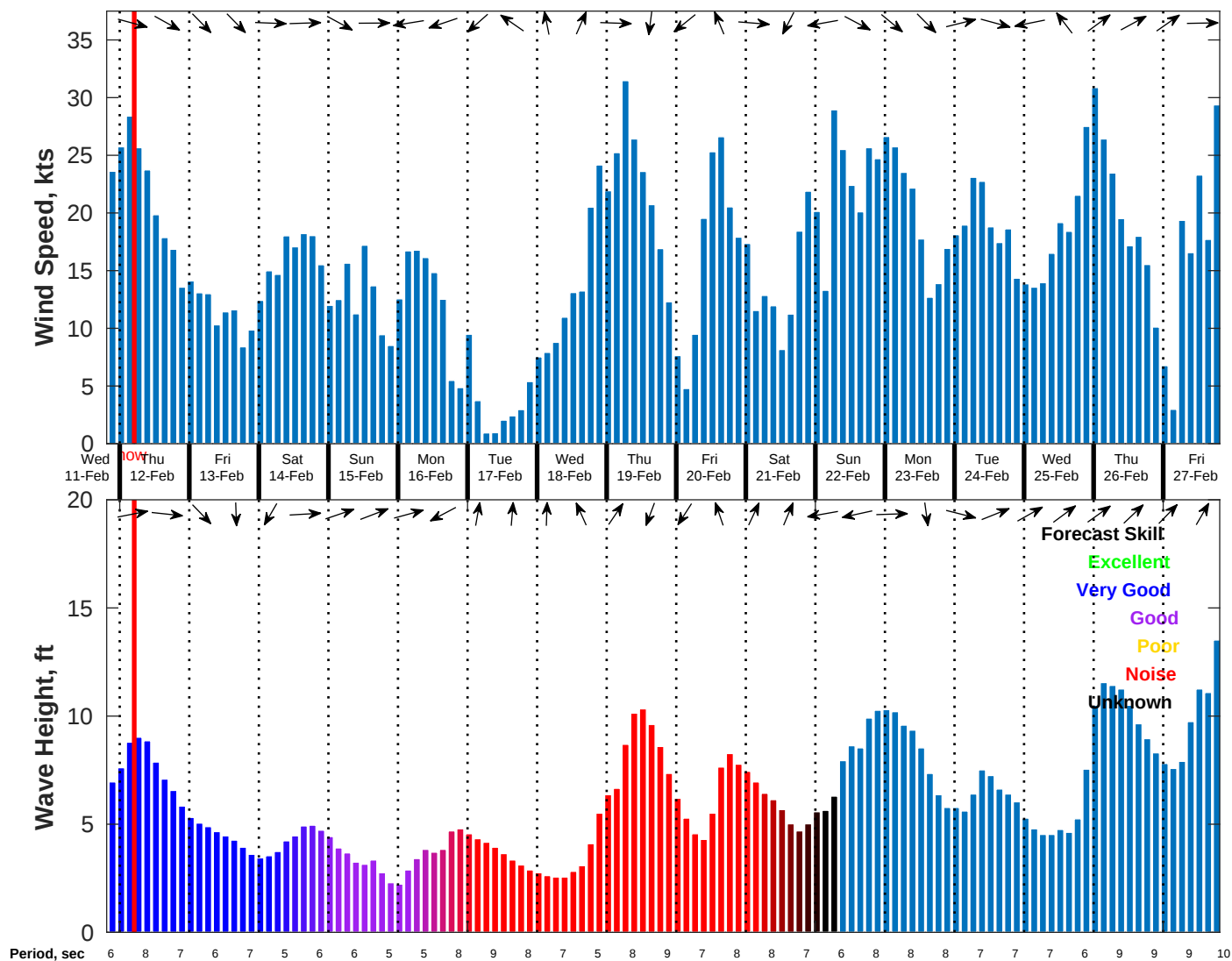
Wind & Wave Forecast for NDBC 44008 from 11-Feb-2026 20:00:00 to 27-Feb-2026 20:00:00
