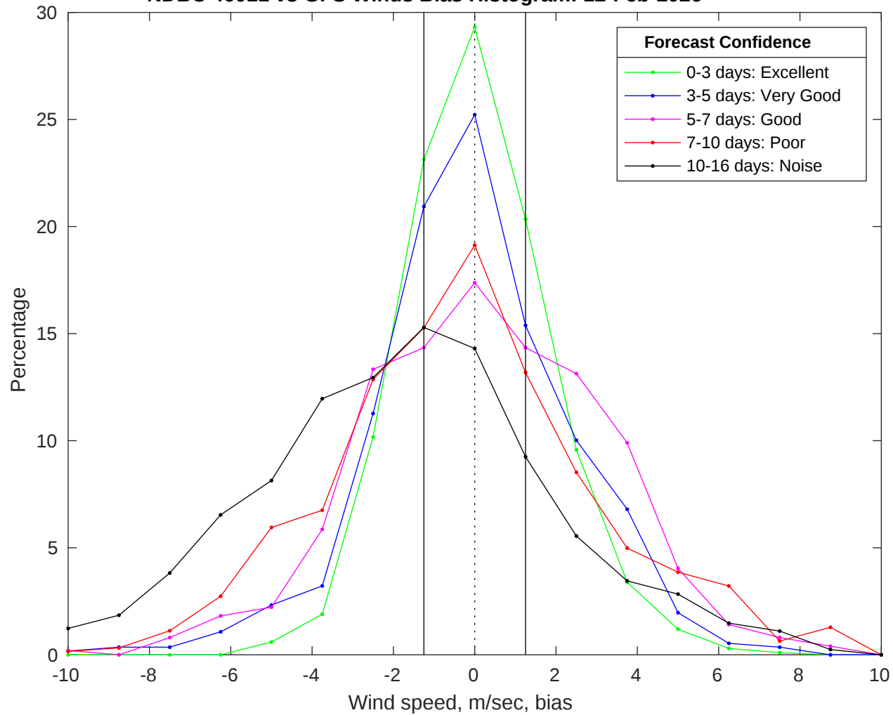
NDBC 46011 vs GFS Winds Bias Histogram: 12-Feb-2026
