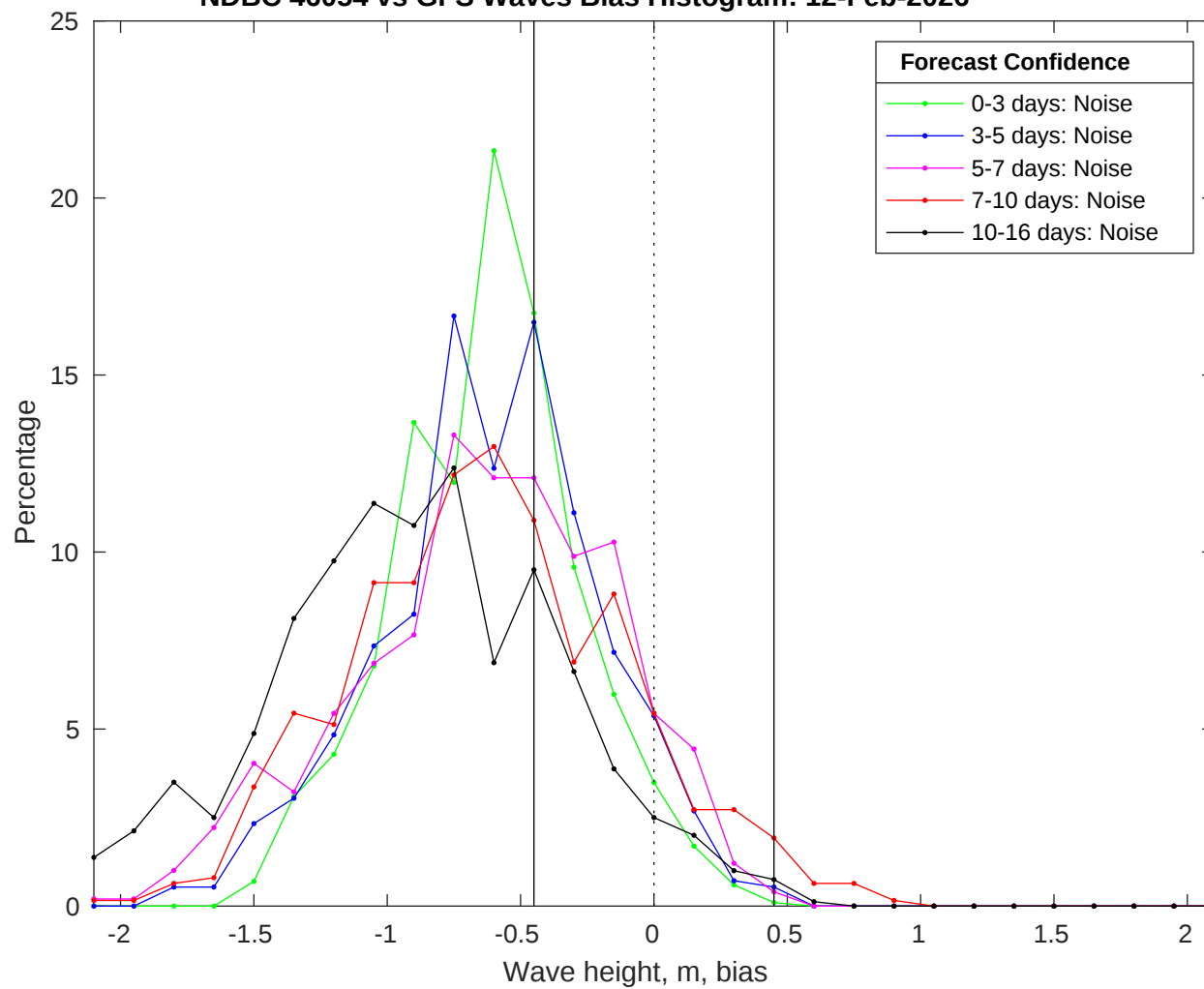
NDBC 46054 vs GFS Waves Bias Histogram: 12-Feb-2026
