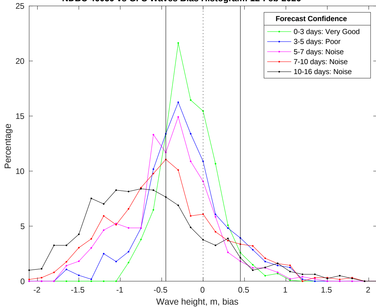
NDBC 46059 vs GFS Waves Bias Histogram: 12-Feb-2026
