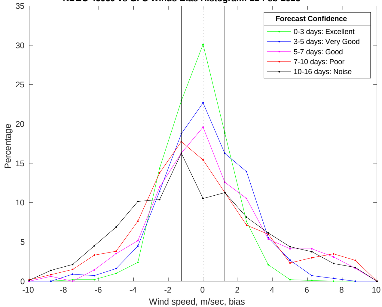
NDBC 46069 vs GFS Winds Bias Histogram: 12-Feb-2026
