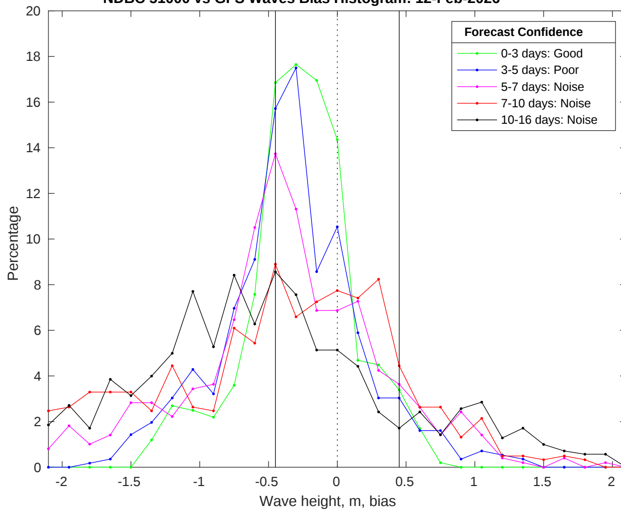
NDBC 51000 vs GFS Waves Bias Histogram: 12-Feb-2026
