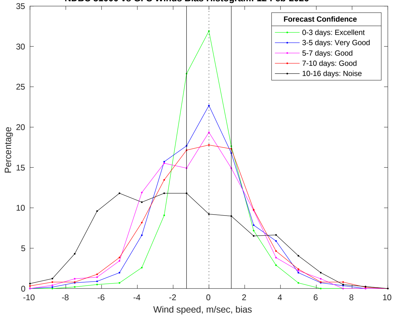
NDBC 51000 vs GFS Winds Bias Histogram: 12-Feb-2026
