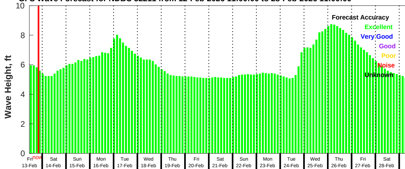
GFS Wave Forecast for NDBC 52211 from 12-Feb-2026 11:00:00 to 28-Feb-2026 11:00:00
