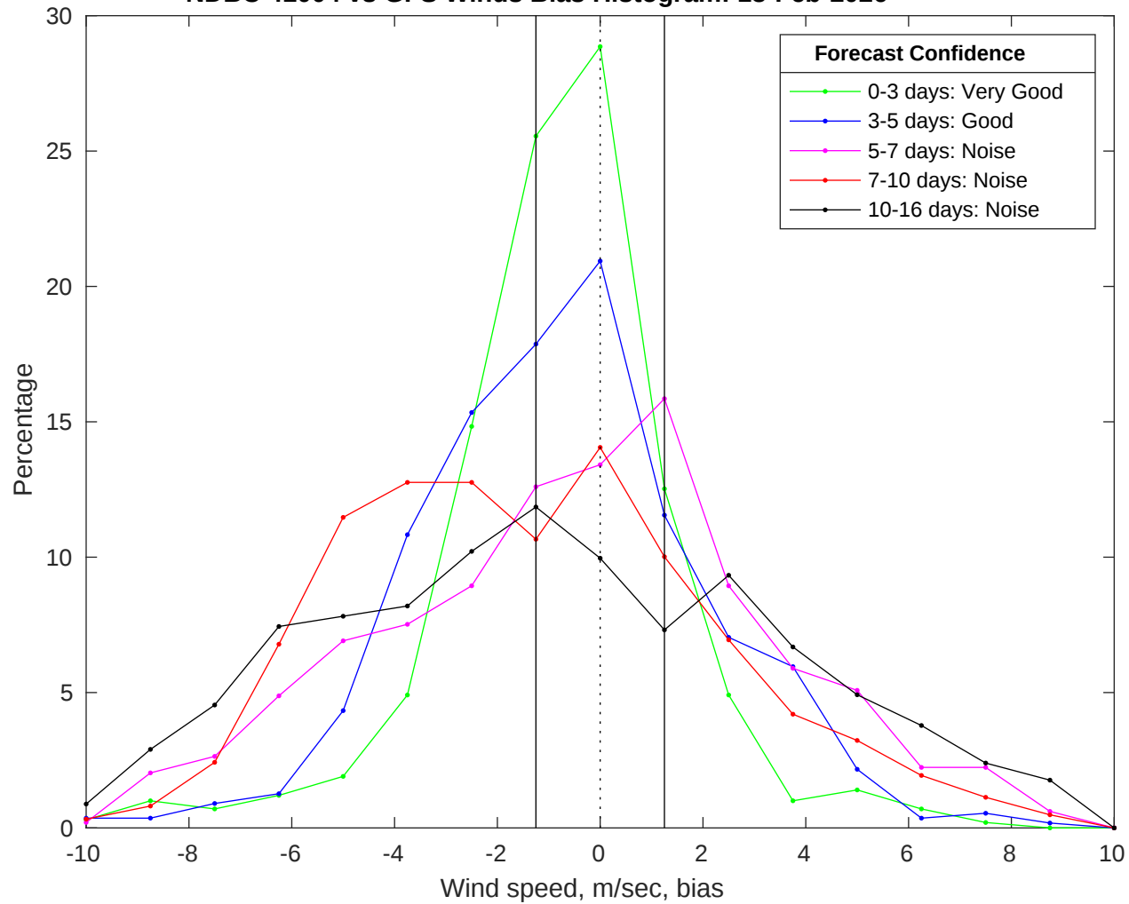
NDBC 41004 vs GFS Winds Bias Histogram: 13-Feb-2026
