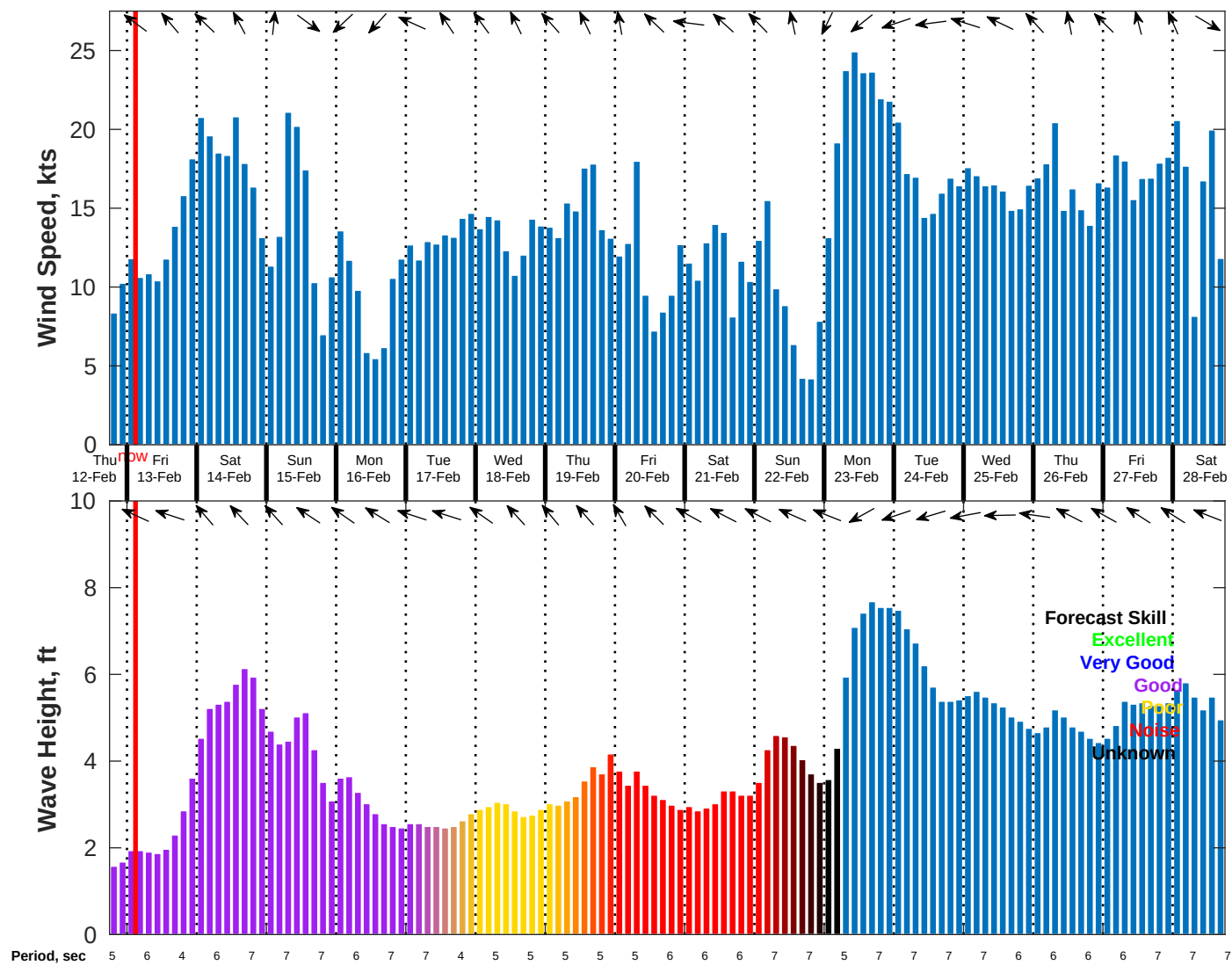
Wind & Wave Forecast for NDBC 42020 from 12-Feb-2026 18:00:00 to 28-Feb-2026 18:00:00
