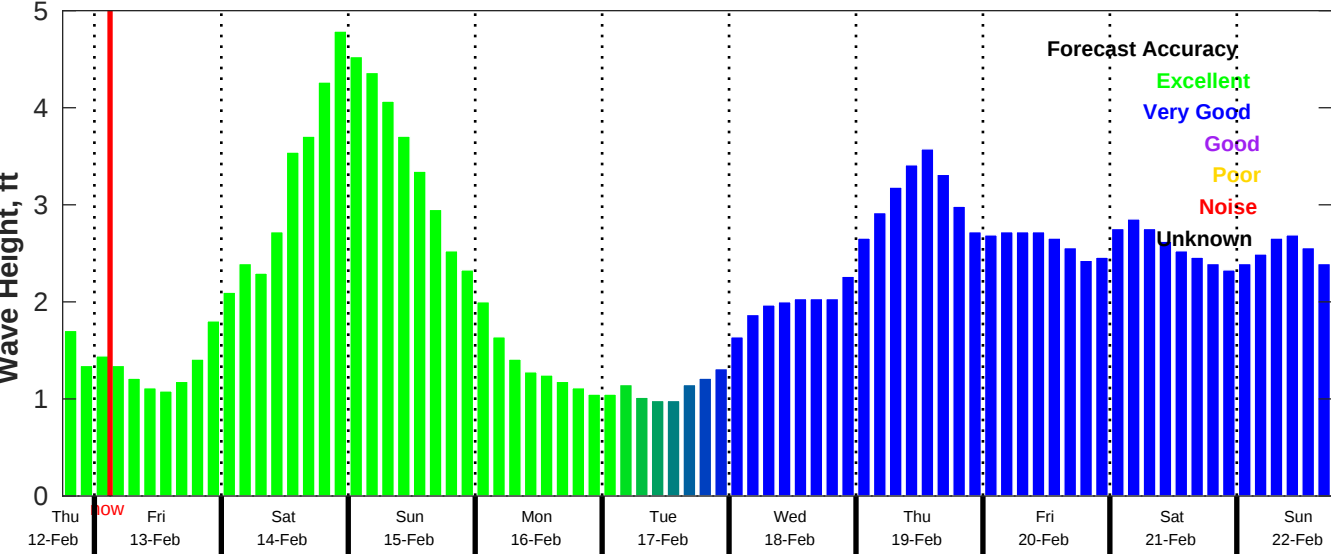
CMEMS Wave Forecast for NDBC 42035 from 12-Feb-2026 18:00:00 to 22-Feb-2026 18:00:00
