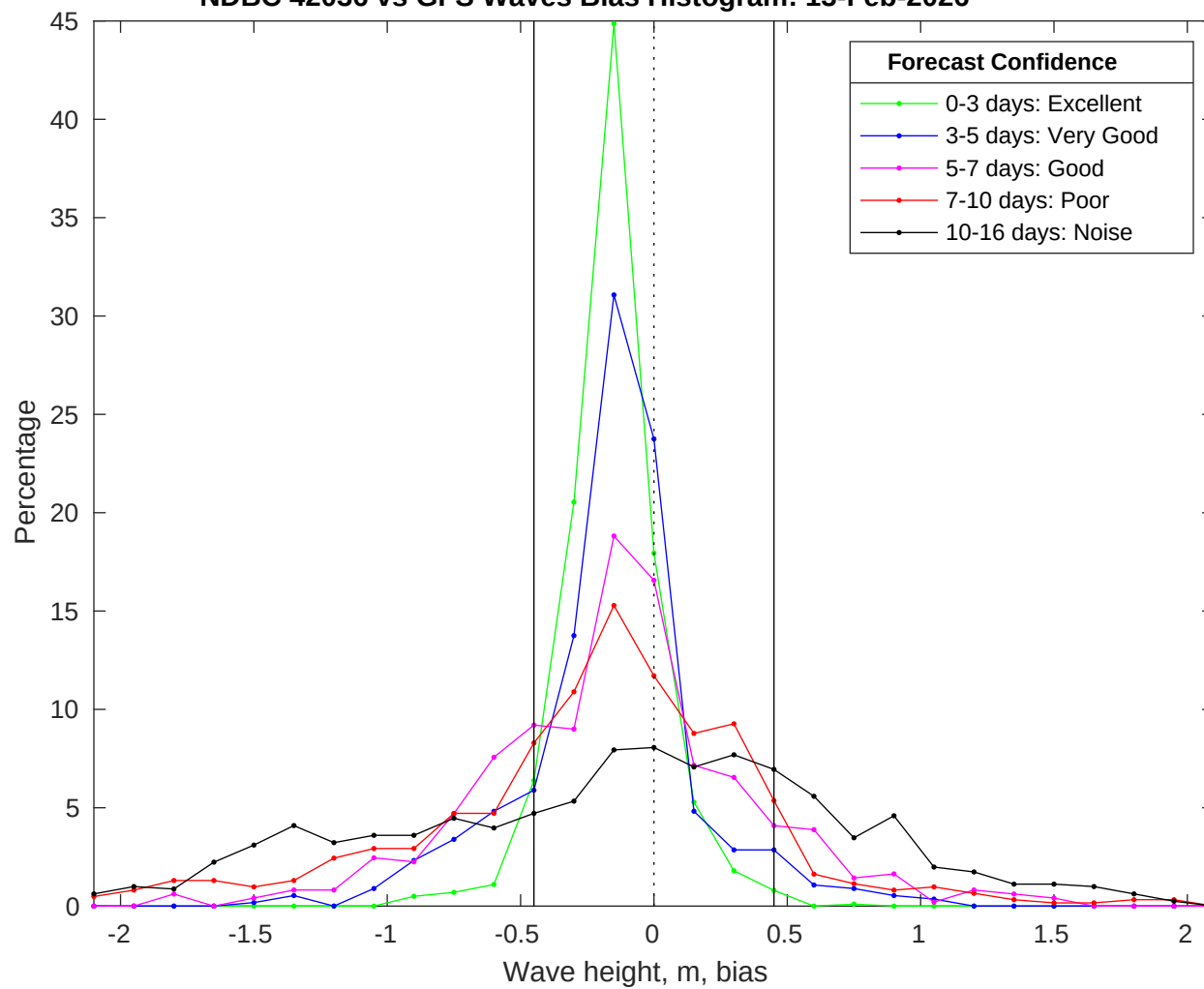
NDBC 42036 vs GFS Waves Bias Histogram: 13-Feb-2026
