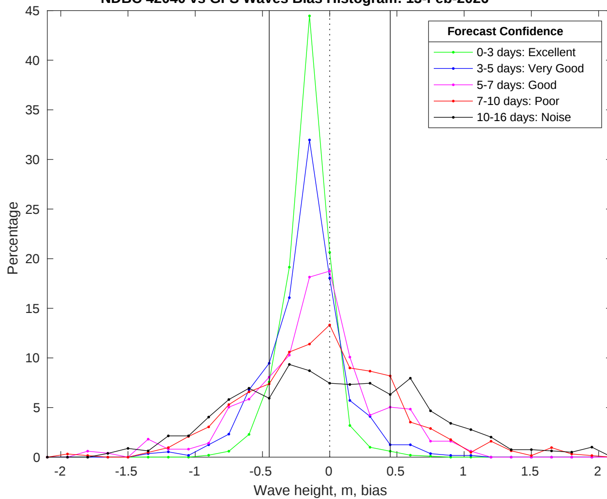
NDBC 42040 vs GFS Waves Bias Histogram: 13-Feb-2026
