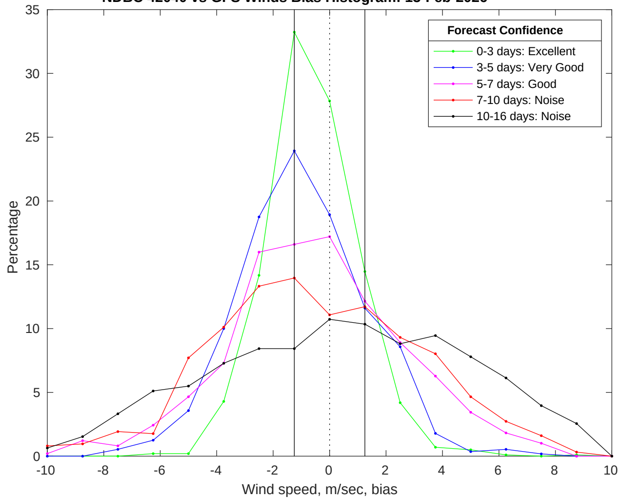
NDBC 42040 vs GFS Winds Bias Histogram: 13-Feb-2026
