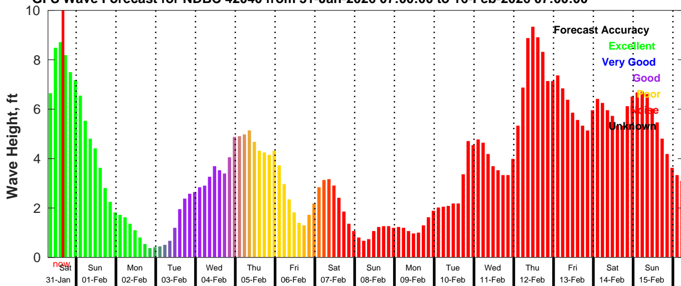
GFS Wave Forecast for NDBC 42040 from 31-Jan-2026 07:00:00 to 16-Feb-2026 07:00:00
