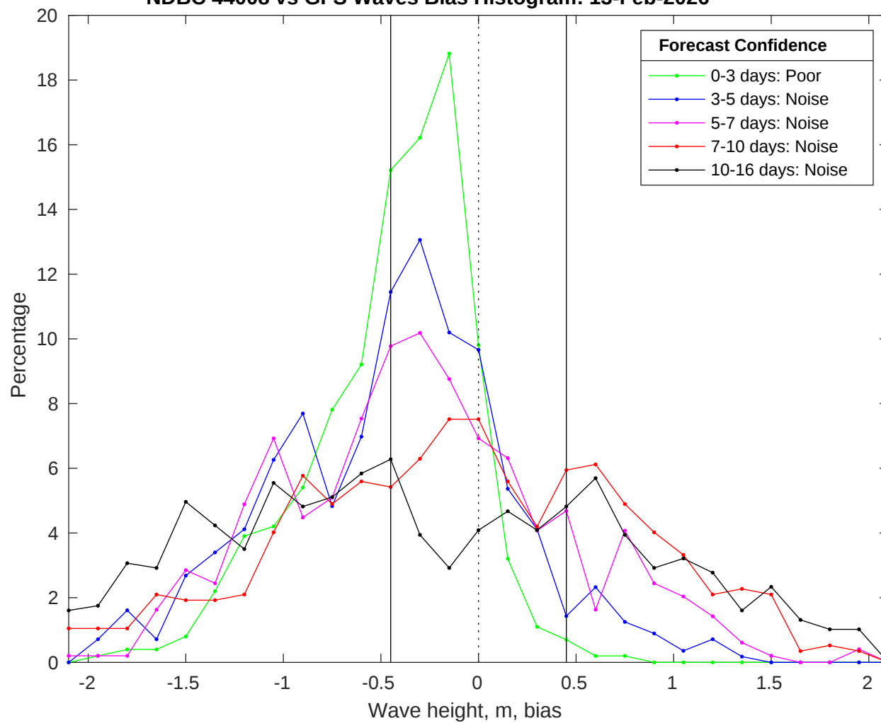
NDBC 44008 vs GFS Waves Bias Histogram: 13-Feb-2026
