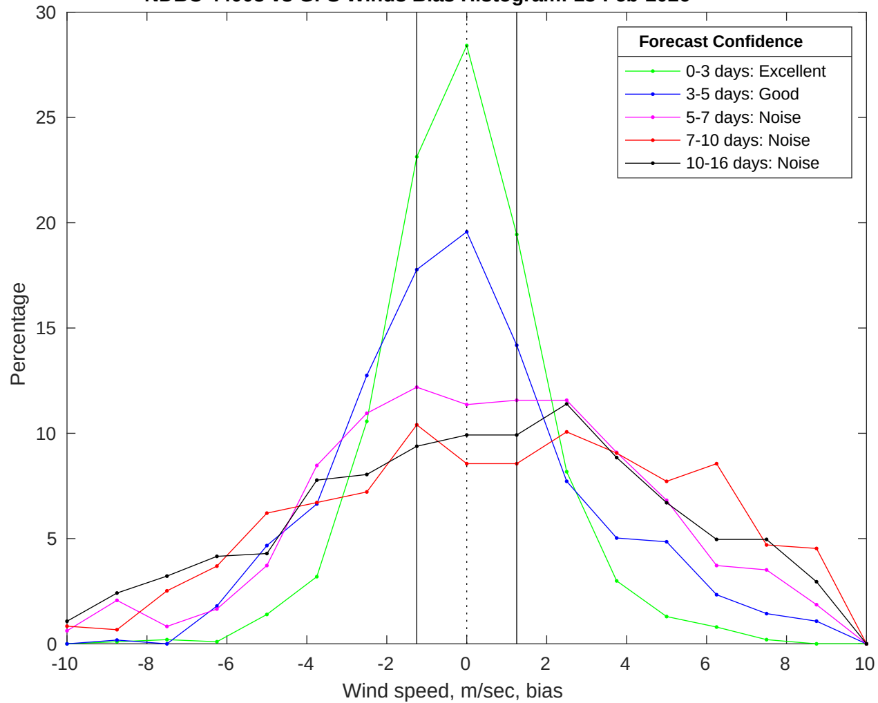
NDBC 44008 vs GFS Winds Bias Histogram: 13-Feb-2026
