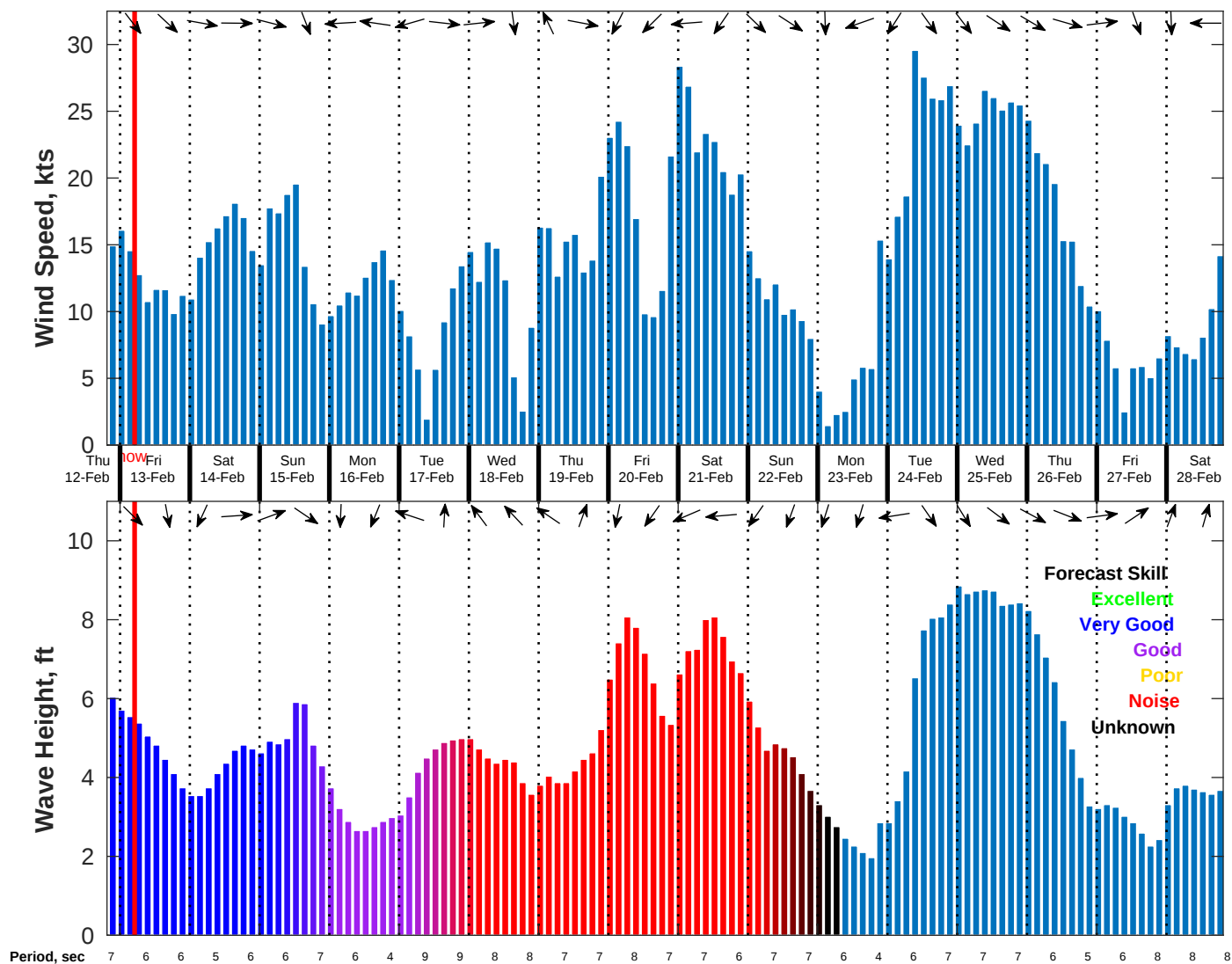
Wind & Wave Forecast for NDBC 44008 from 12-Feb-2026 20:00:00 to 28-Feb-2026 20:00:00
