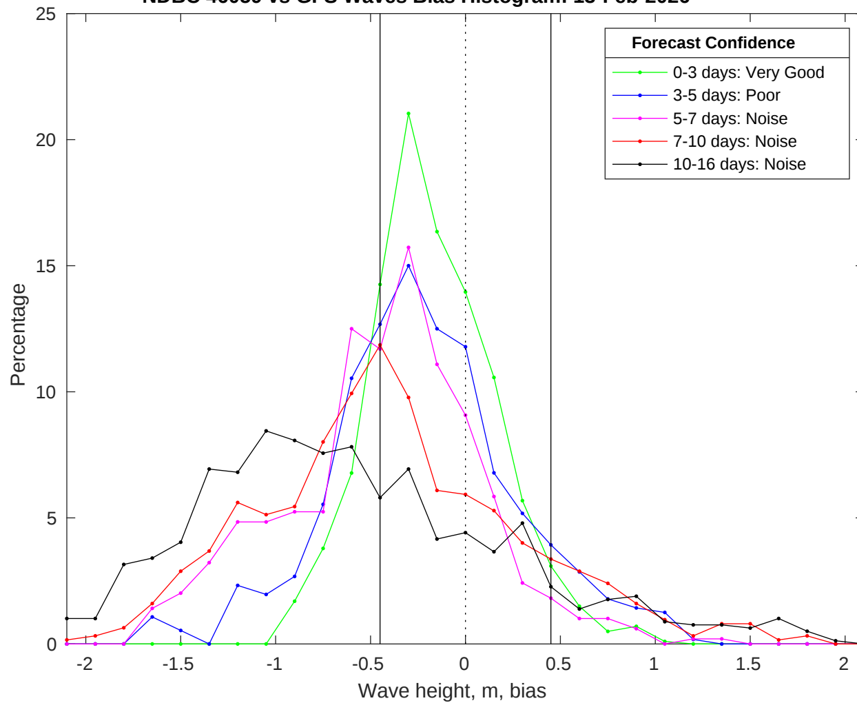
NDBC 46059 vs GFS Waves Bias Histogram: 13-Feb-2026
