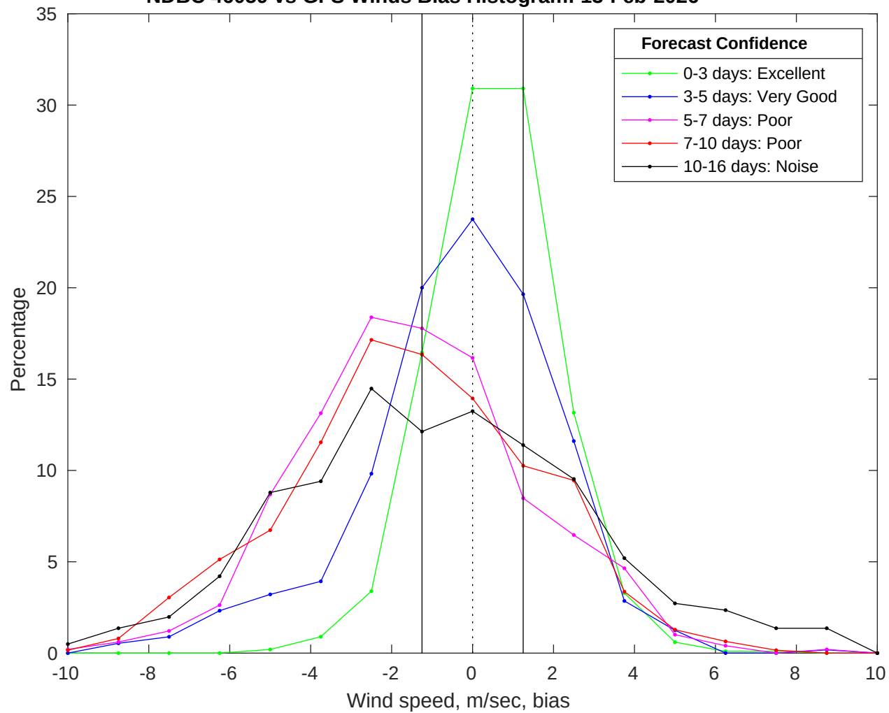
NDBC 46059 vs GFS Winds Bias Histogram: 13-Feb-2026
