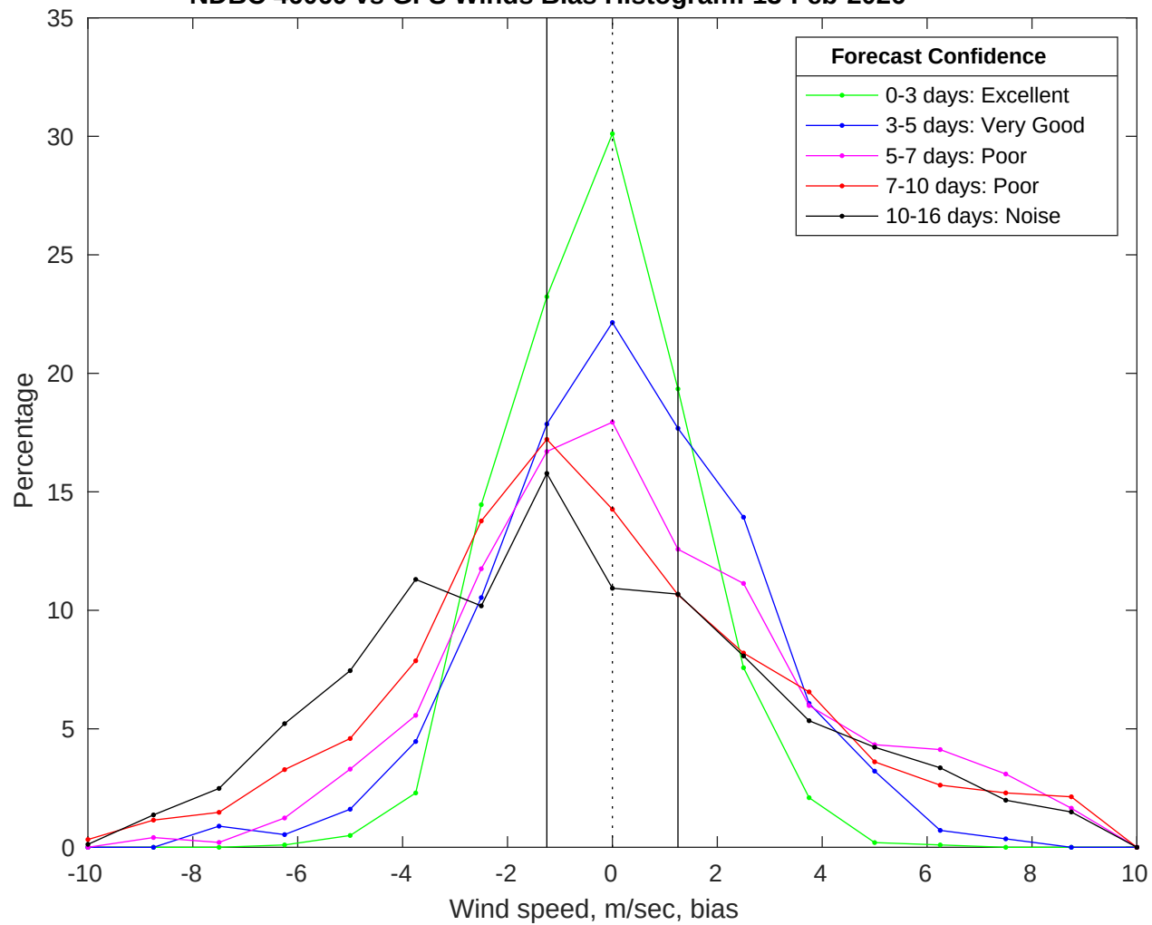
NDBC 46069 vs GFS Winds Bias Histogram: 13-Feb-2026
