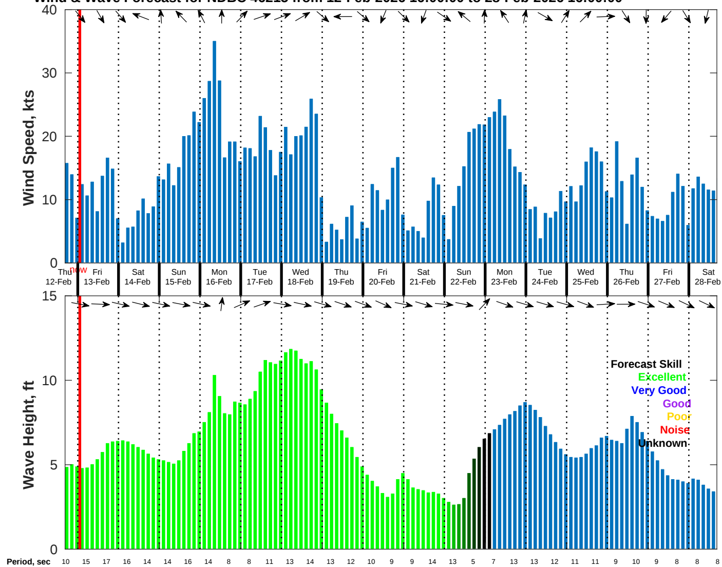
Wind & Wave Forecast for NDBC 46215 from 12-Feb-2026 16:00:00 to 28-Feb-2026 16:00:00
