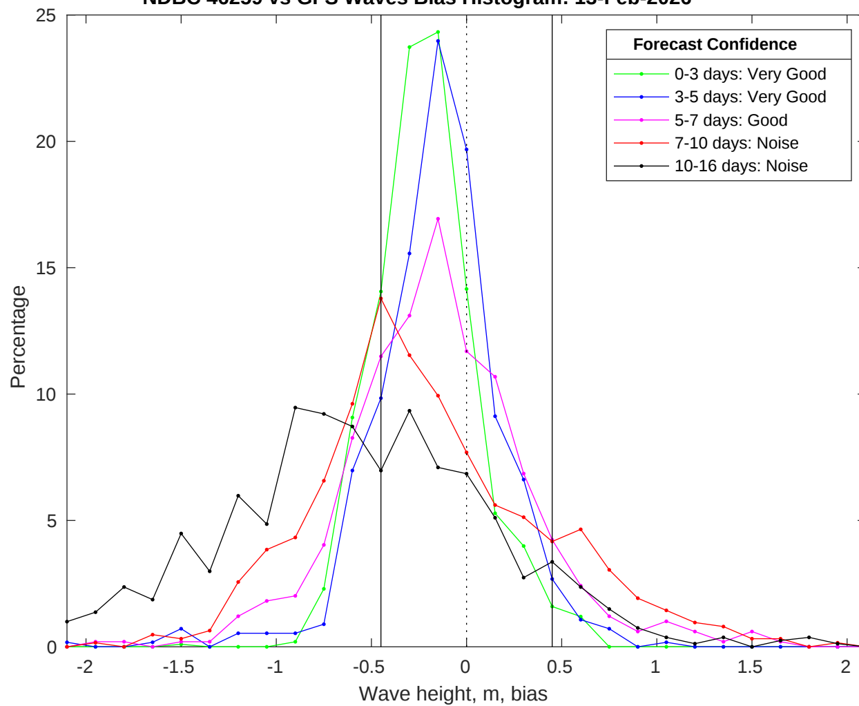
NDBC 46259 vs GFS Waves Bias Histogram: 13-Feb-2026
