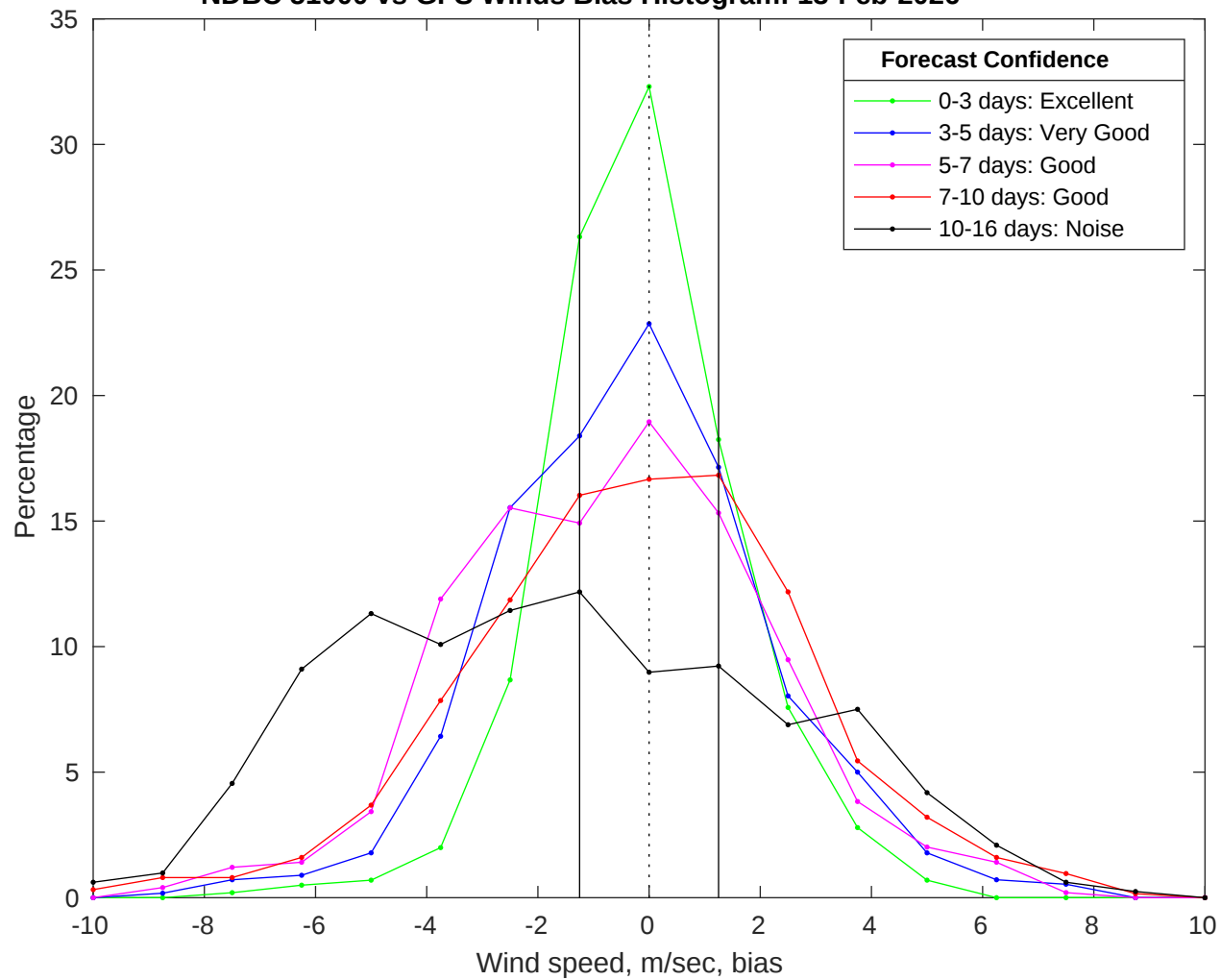
NDBC 51000 vs GFS Winds Bias Histogram: 13-Feb-2026
